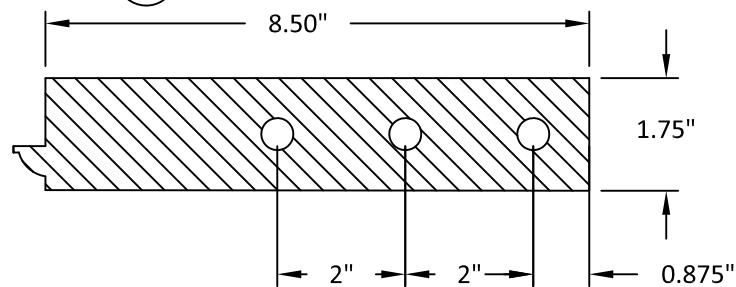
13 TOP RAIL
