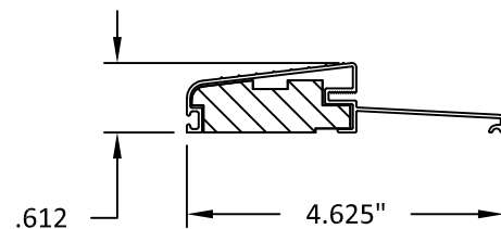
12 OUTSWING THRESHOLD
