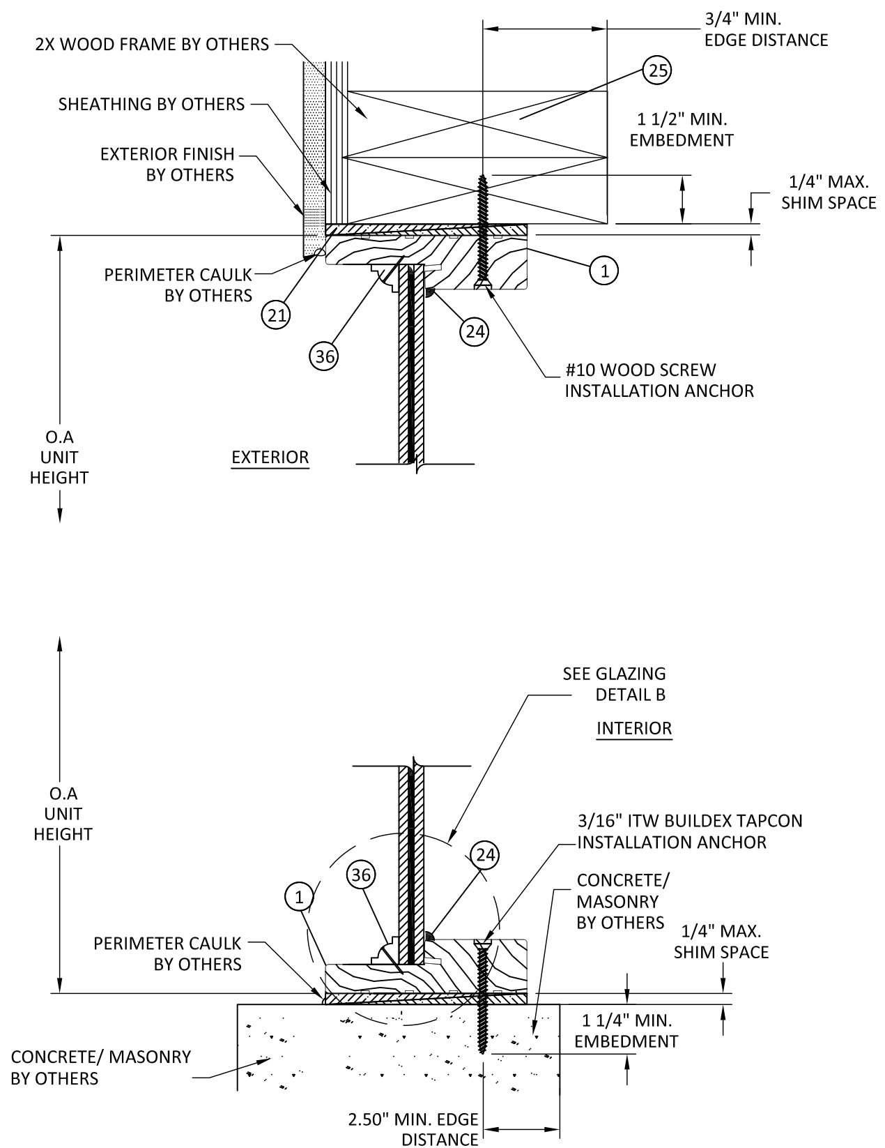
F 5 VERTICAL SECTION OUTSWING DIRECT SET SIDELITE TYP.
