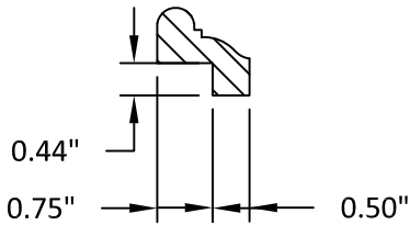
16 GLASS STOP/TRIM
