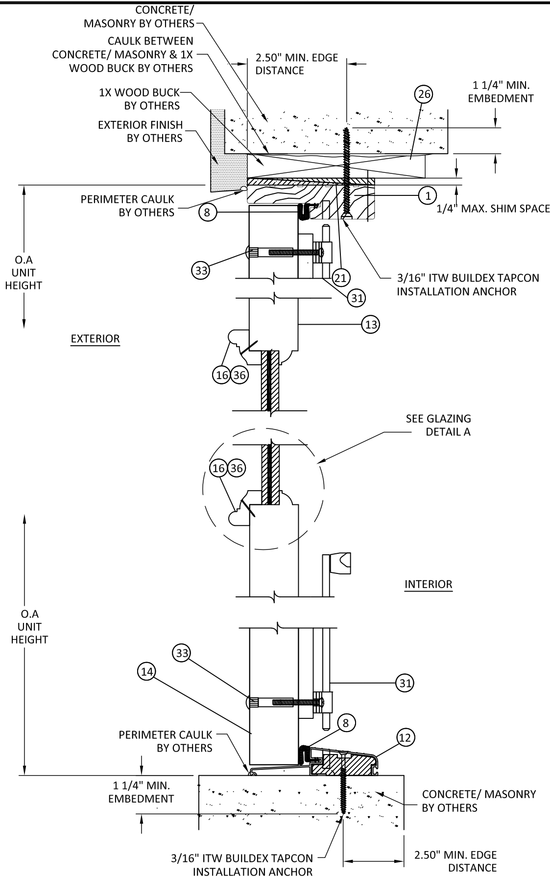
B 3 VERTICAL SECTION OUTSWING ACTIVE/INACTIVE DOOR TYP.
