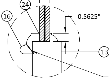
GLAZING DETAIL A
