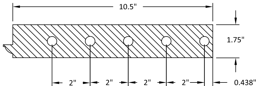
14 BOTTOM RAIL
