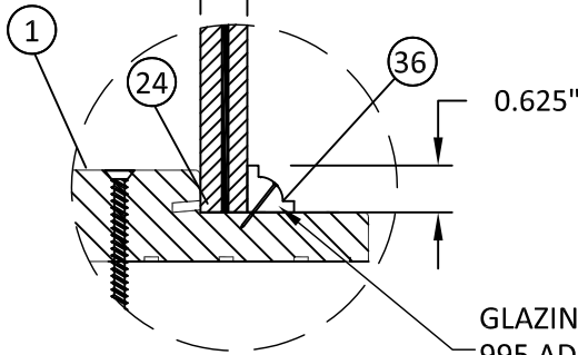
GLAZING DETAIL B
