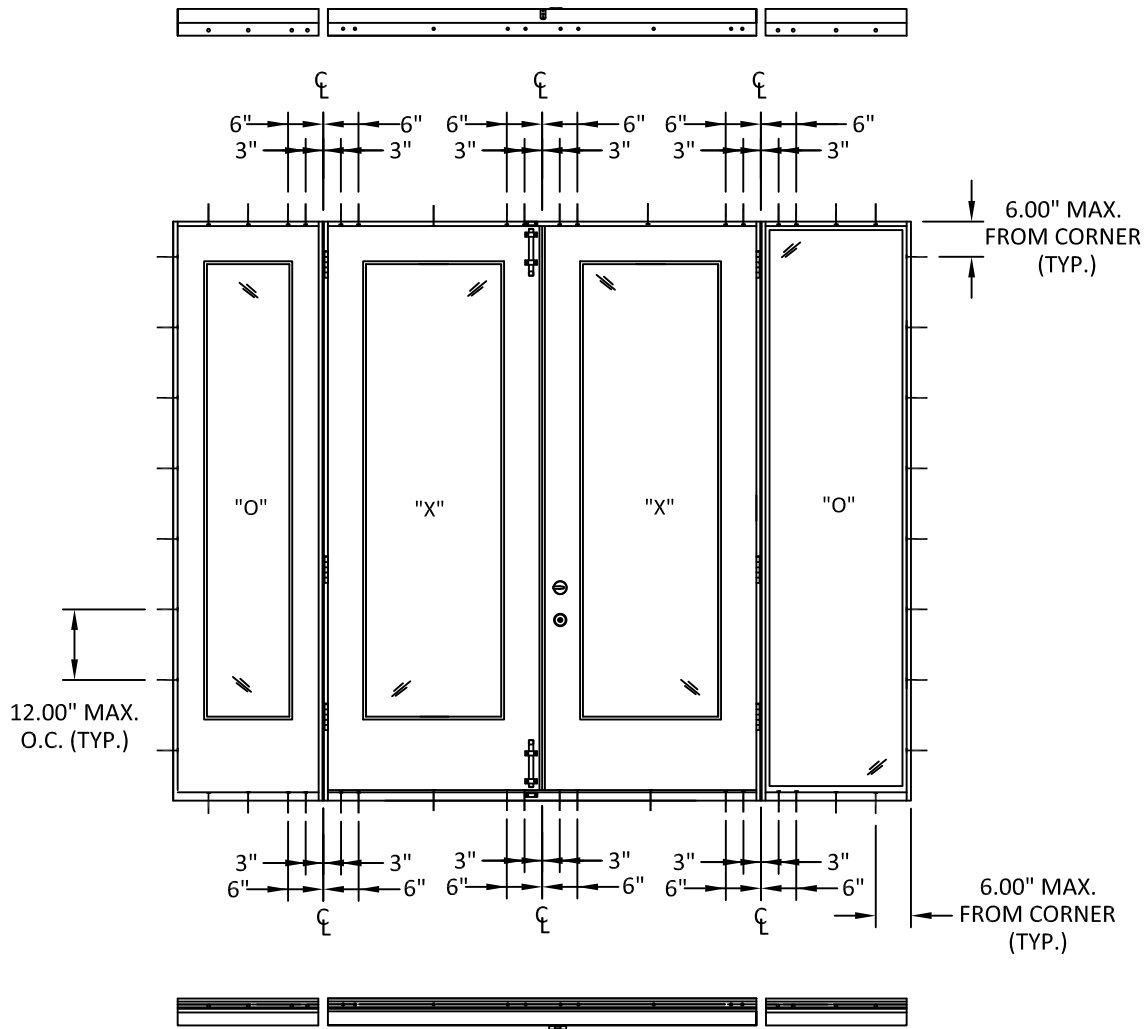
ANCHOR LAYOUT
