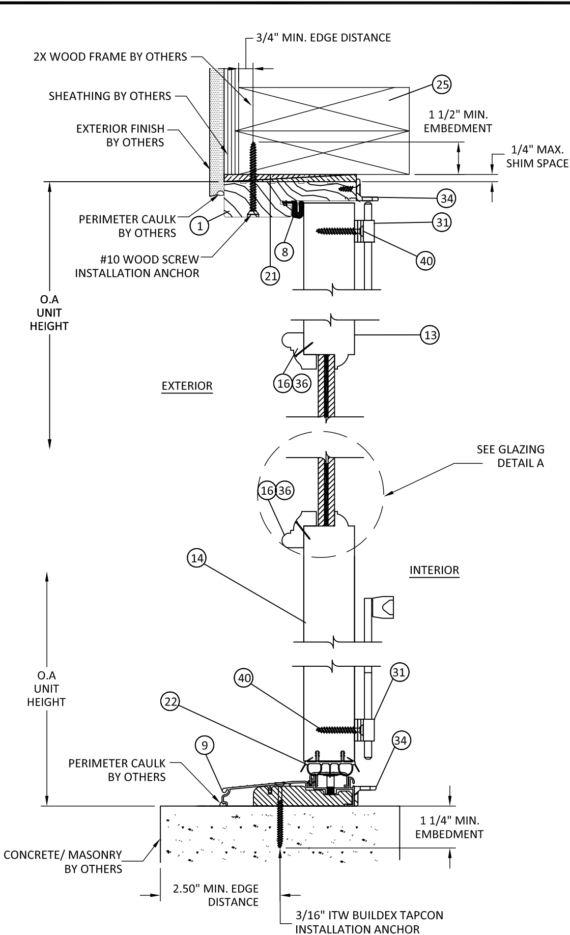
A 3 VERTICAL SECTION INSWING ACTIVE DOOR TYP.
