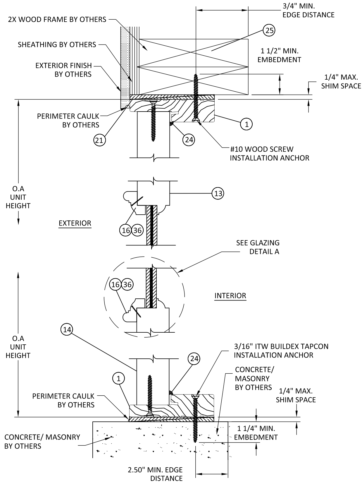
E 5 VERTICAL SECTION OUTSWING FIXED SASH SIDELITE TYP.
