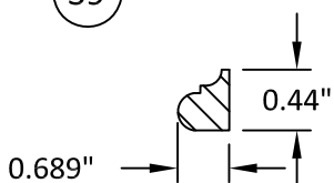
39 EXT. PANEL MOLDING
