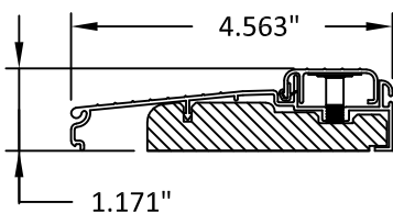
9 INSWING THRESHOLD
